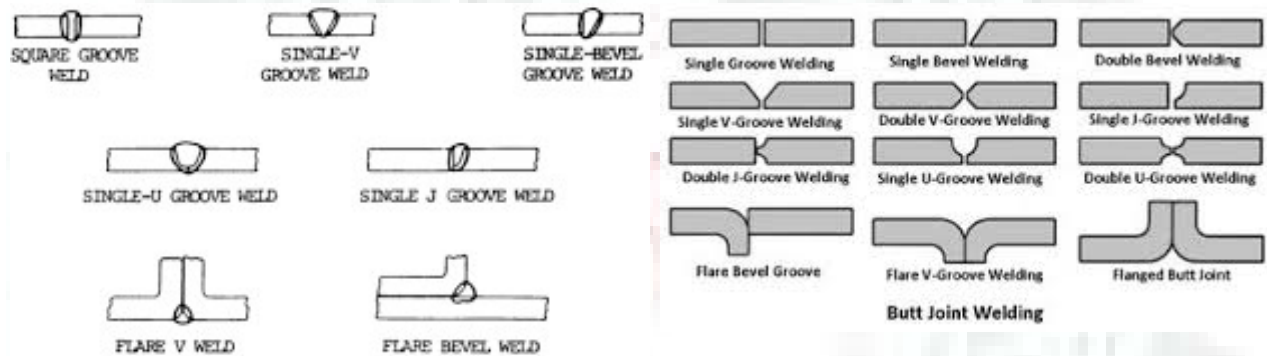
Figure 6-25. Basic groove welds.
