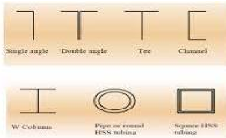
Different Shape Compression member
